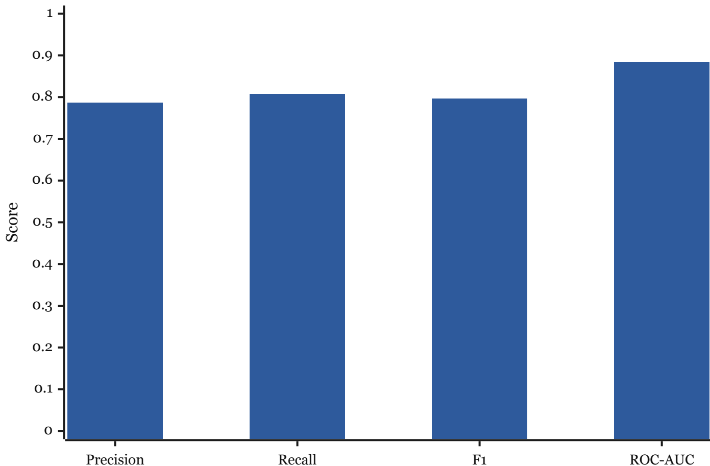
ML metrics — synthetic pipeline validation (n_test = 4500)
